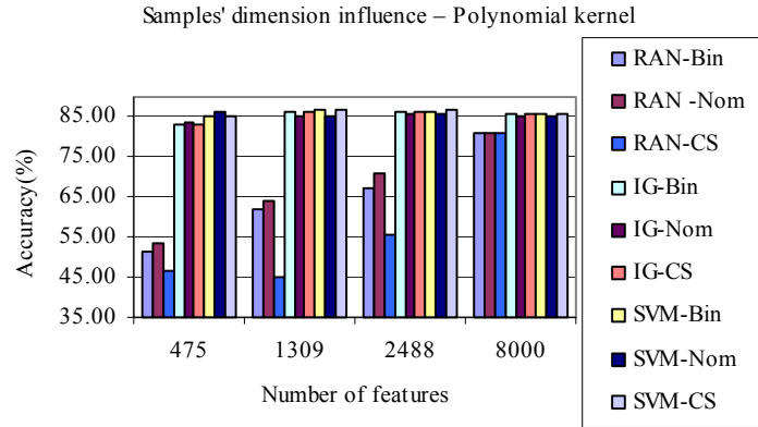
Fig. 1. Influence of the number of features on the classification accuracy using Polynomial kernel with degree equal to 2 (BIN – means Binary representation, Nom – nominal representation and CS – Cornel Smart representation)
