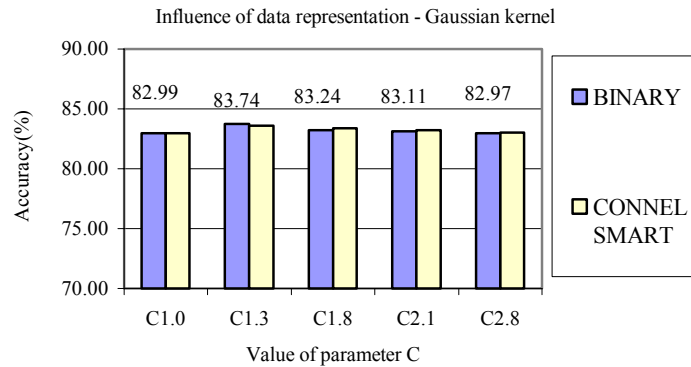
Fig. 4. Influence of data representation and parameter C for Gaussian kernel
